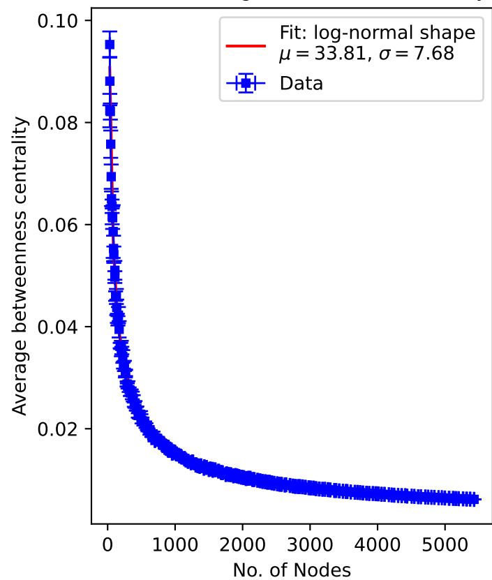
Log-Normal Fit and Plot of Nodes vs Average betweenness centrality
