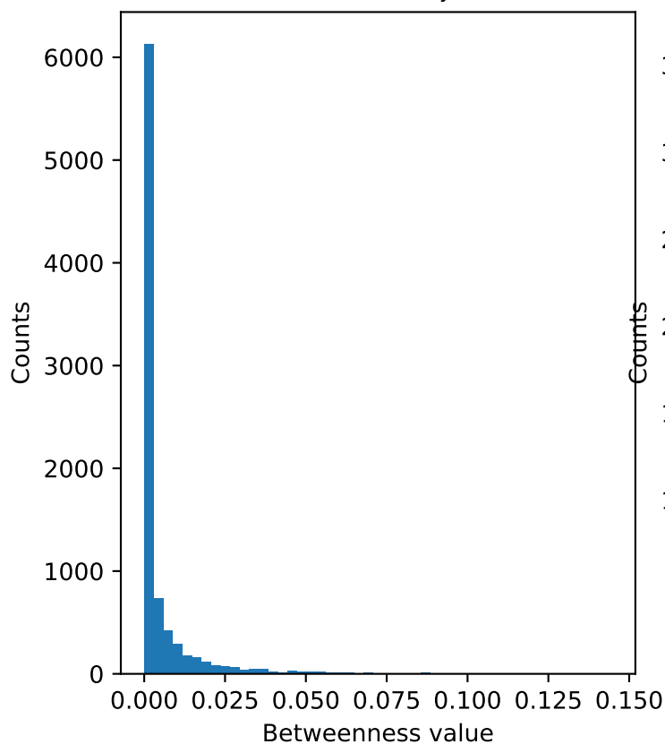
Betweenness Centrality: \sigma=0.011
