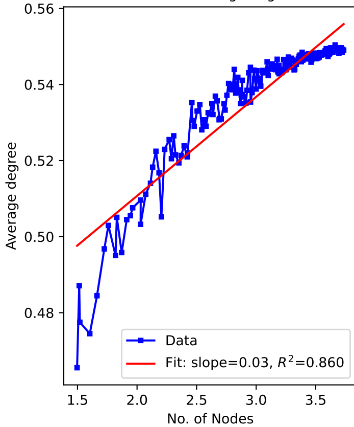
Log-Log Plot of Nodes vs Average degree
