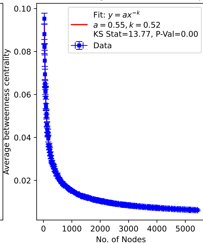
Power Law Fit and Plot of Nodes vs Average betweenness centrality
